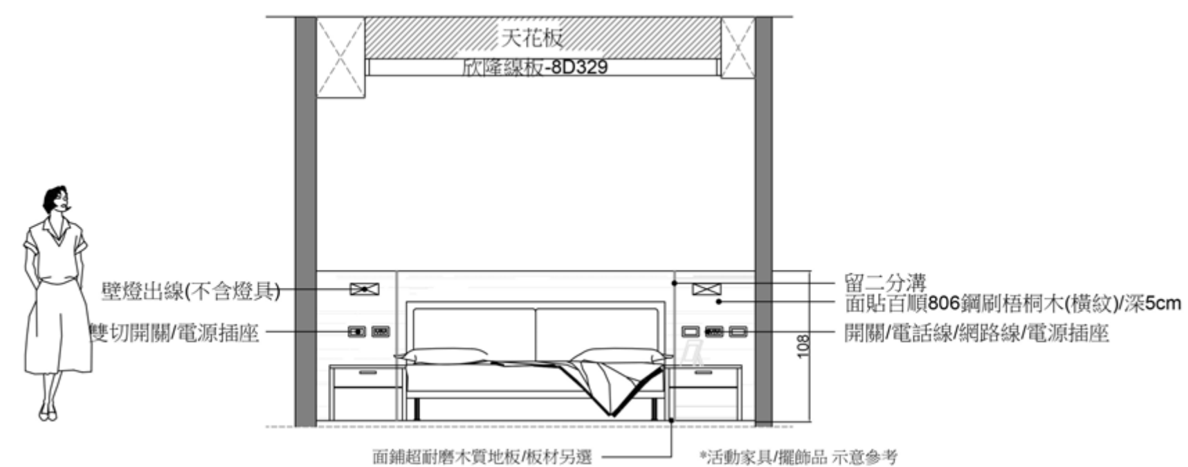
[ Master room Headboard Elevation ]
