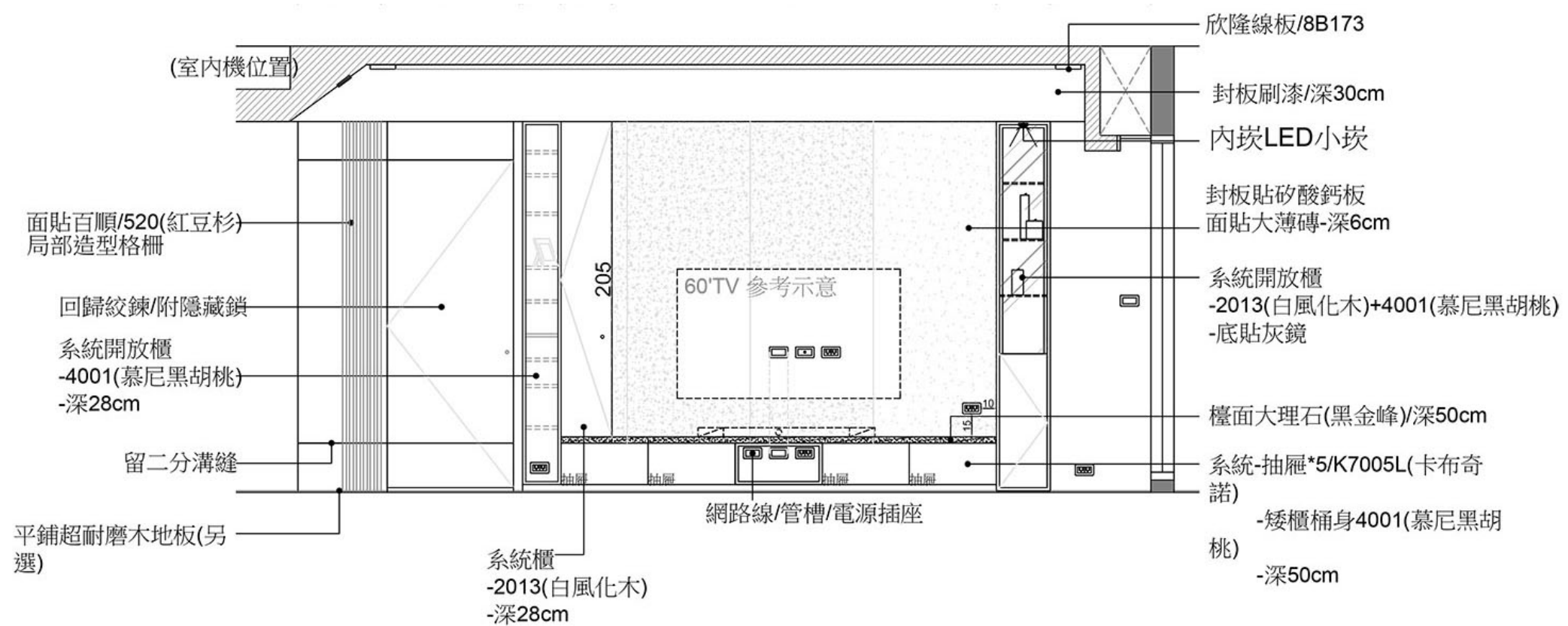
[ TV Wall Elevation 1:30 ]
